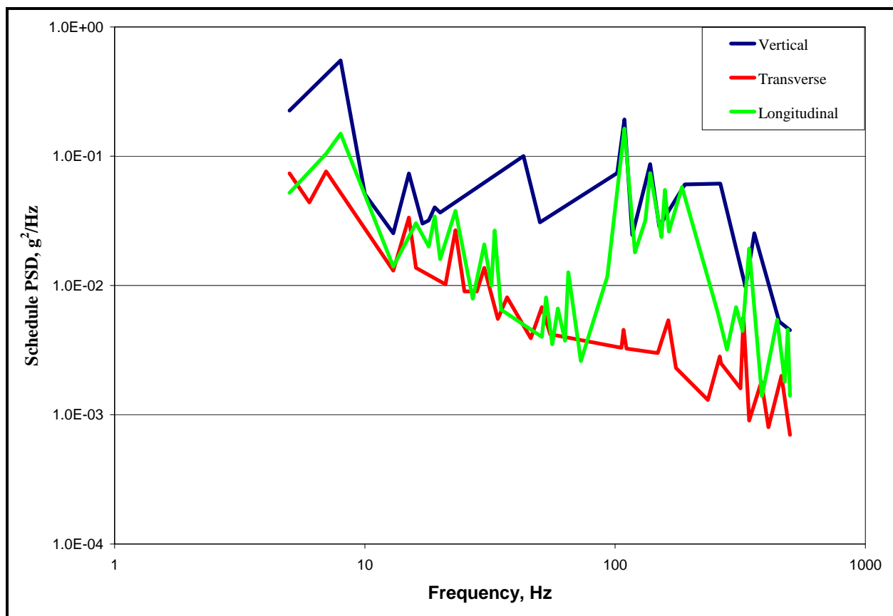
Figure 514.6C-2 – Category 4 – Composite two-wheeled trailer vibration exposure.
