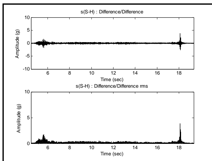
Figure 525A-9c. Time Trace of Difference of the Differences ((S) – (H))
