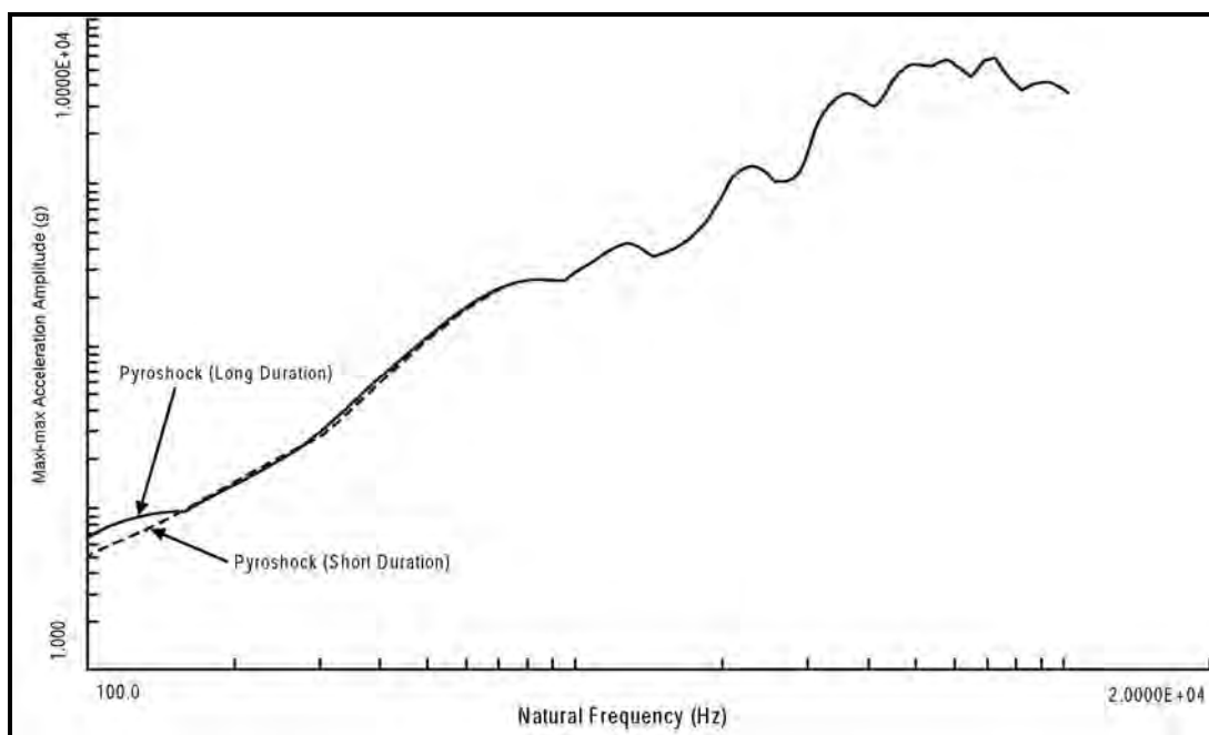
Figure 517.1-4. Acceleration maximax SRS – (long vs short duration).
