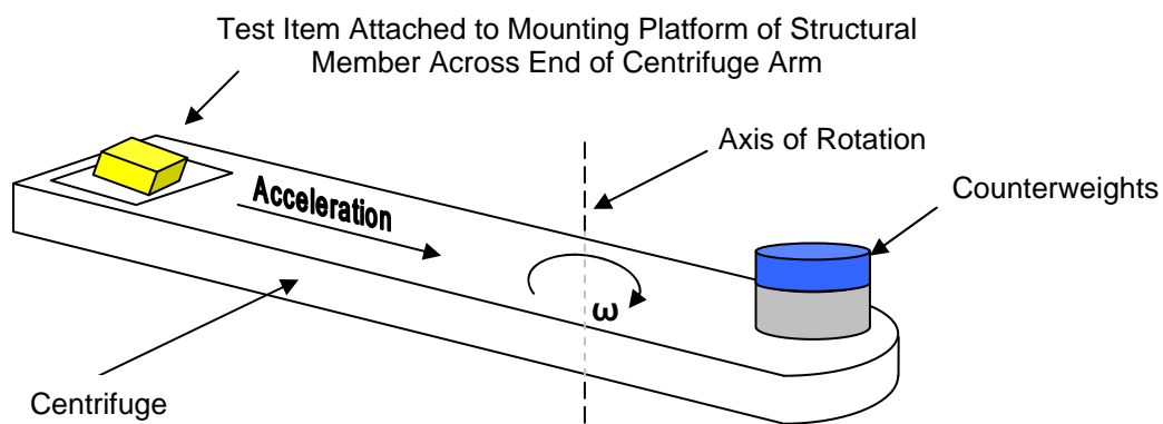
Typical Installation
