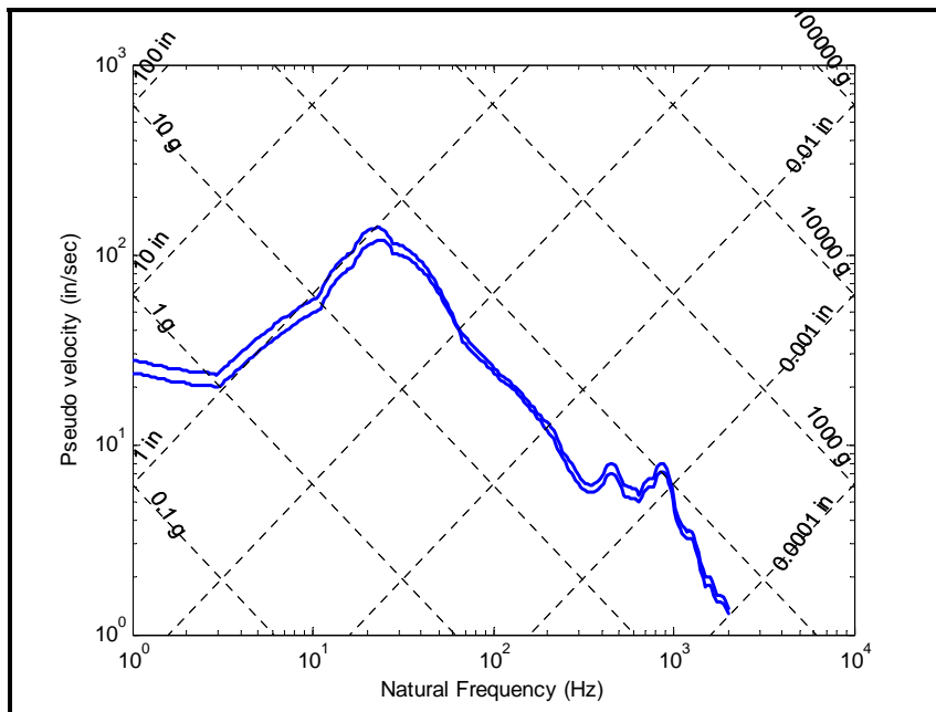
Figure 525A-24a Composite pseudo-velocity maximax pseudo-velocity SRS for r and c.
