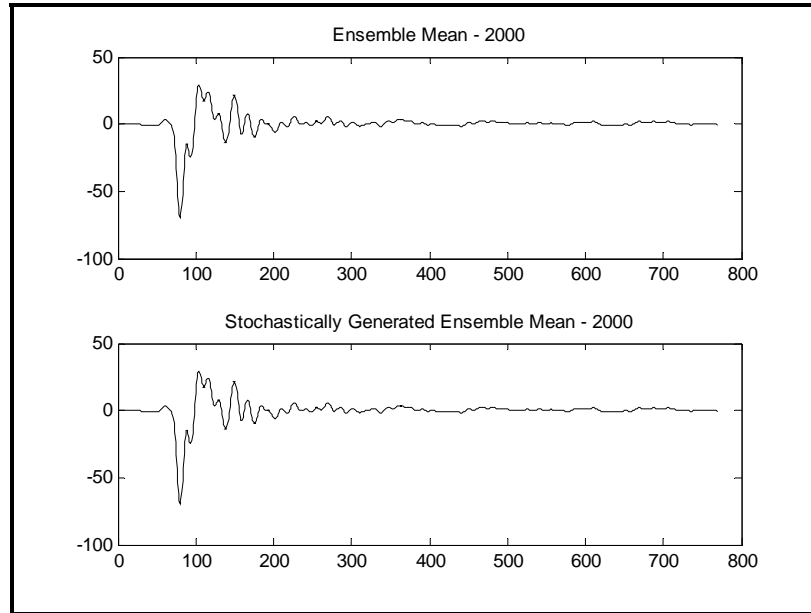
Figure 519.6B-8a. Ensemble and stochastically generated pulse ensemble deterministic component (2000 r/min).
