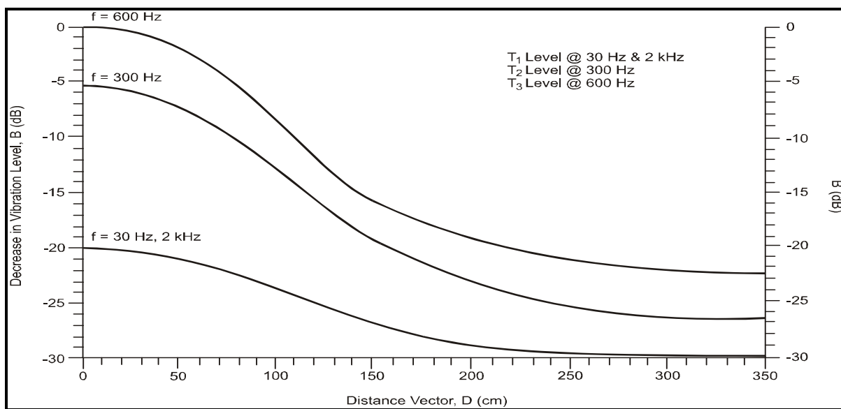
FIGURE 519.6D-7. Decrease in vibration level with vector distance from gun muzzle.
