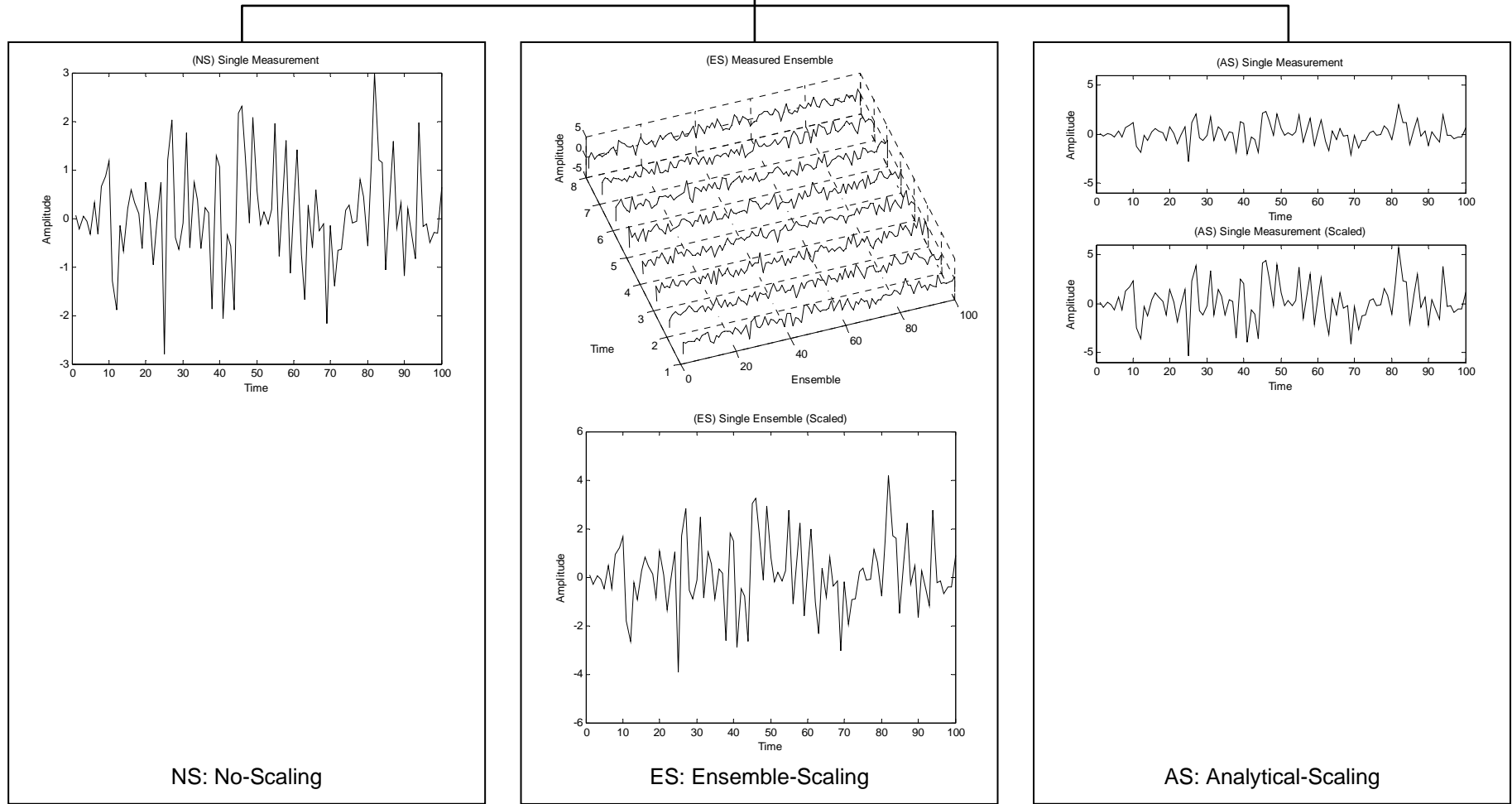
Figure 525-1. Basic TWR test modes as related to time trace scaling.
