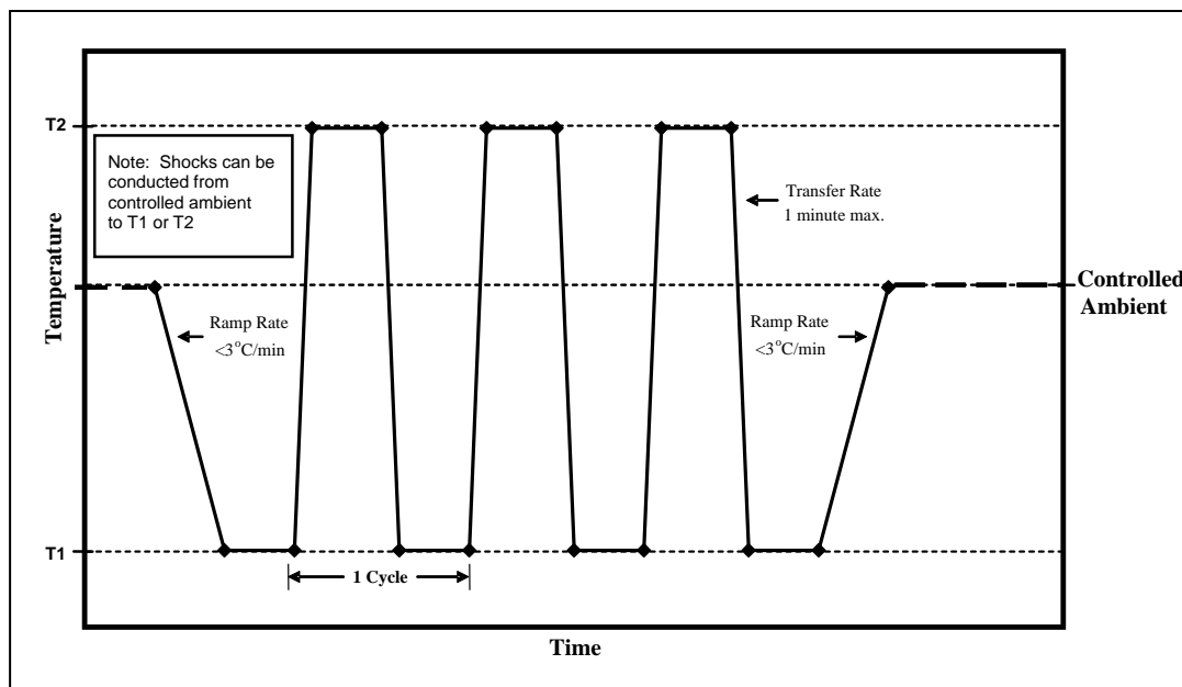
Figure 503.5-3. Multi-cycle shocks.
