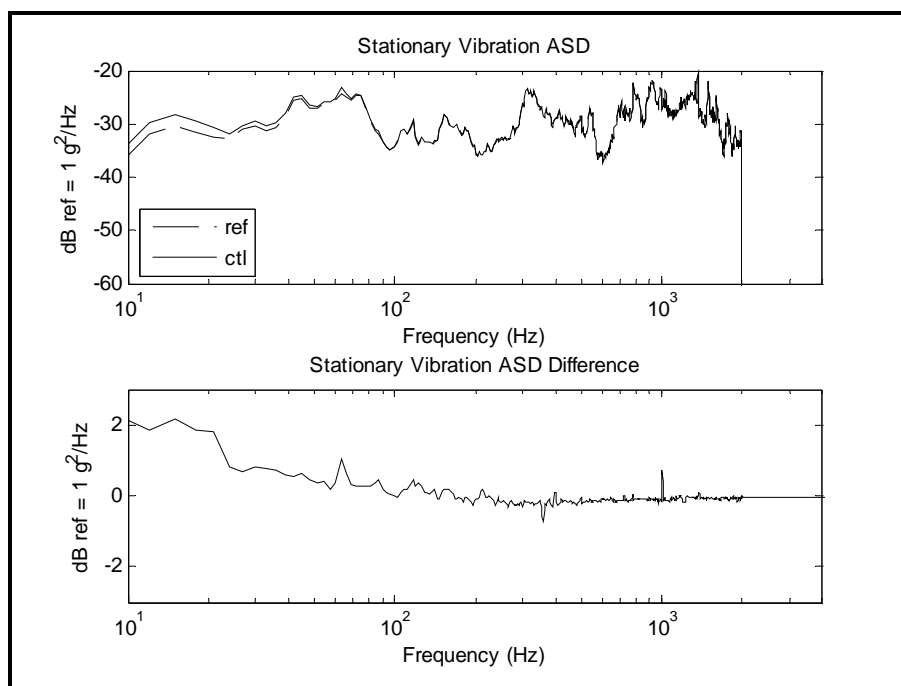
Figure 525A-18a. Composite ASD estimates for r and c.
