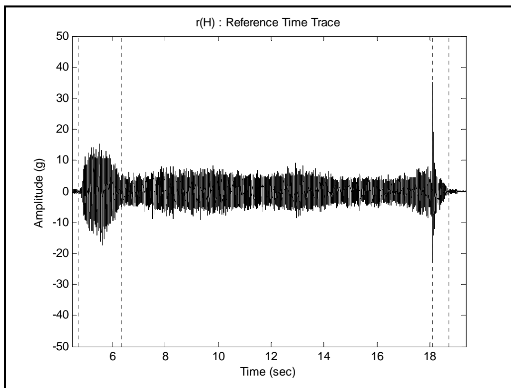
Figure 525A-5. Time trace segment identification from previously truncated reference time trace.
