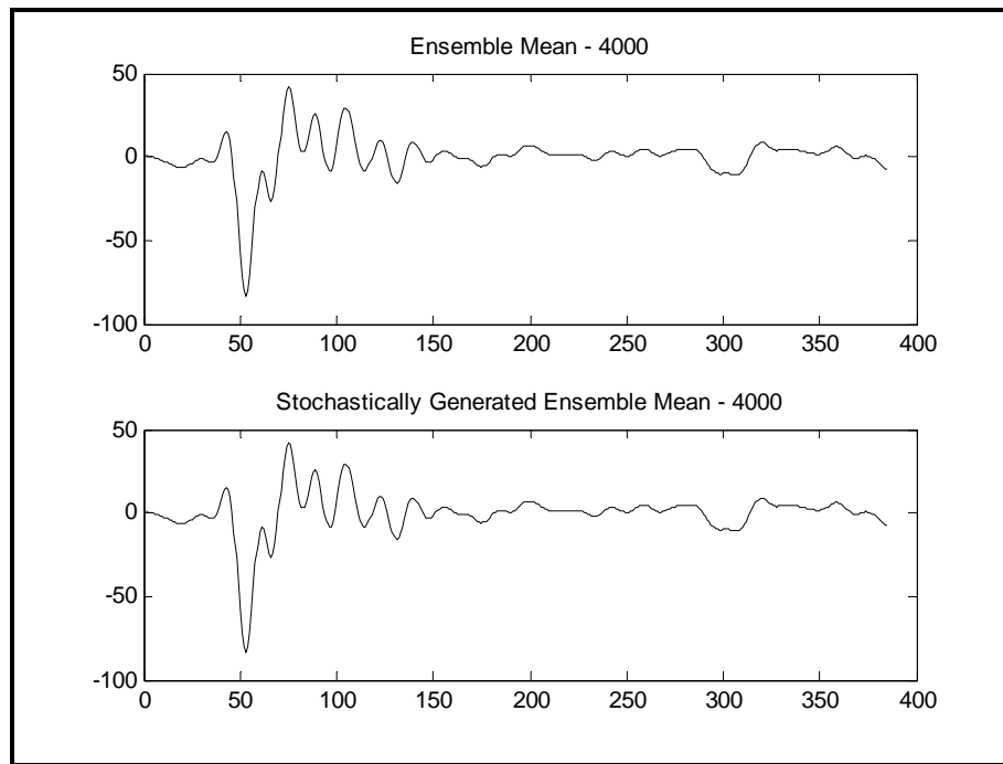
Figure 519.6B-8b. Ensemble and stochastically generated pulse ensemble deterministic component (4000 r/min).
