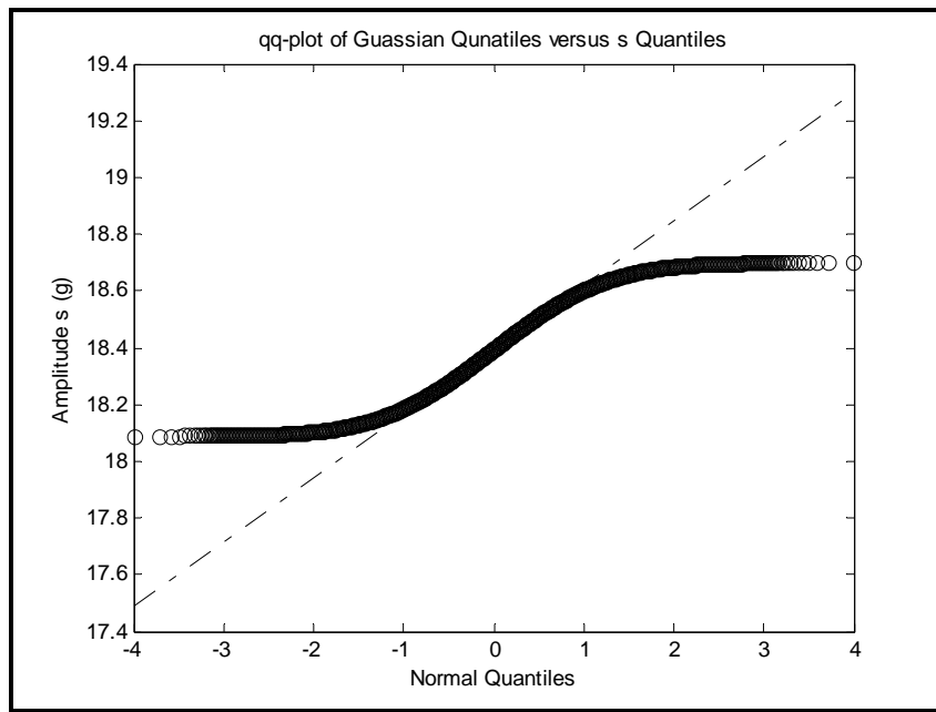
Figure 525A-23. Shock q-q plot for s versus Gaussian
