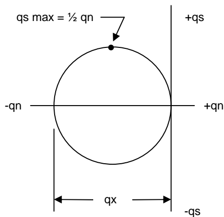
Mohr's Circle for Simple Compression
