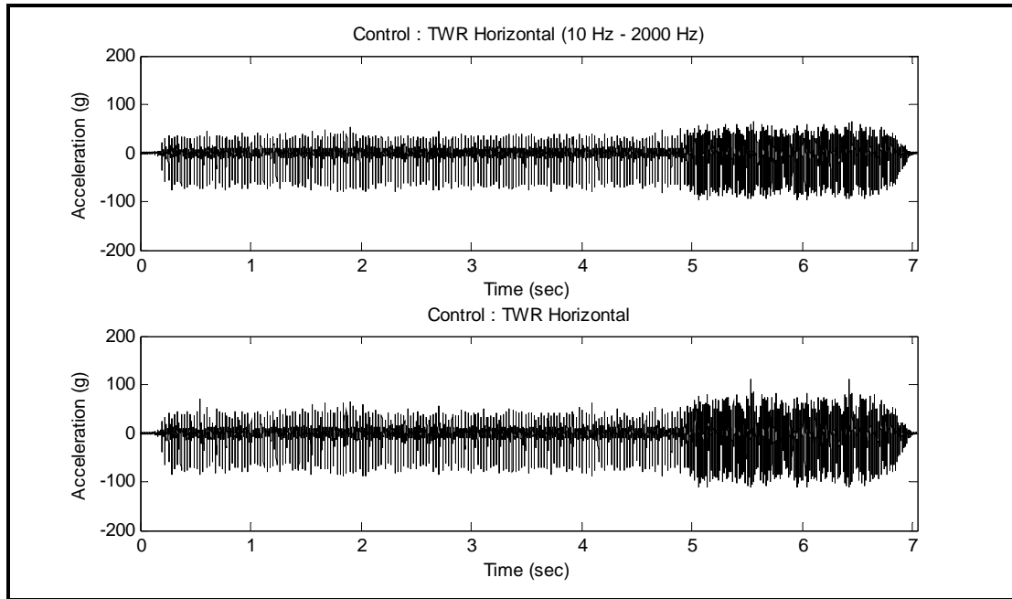
Figure 519.6A-3. Bandlimited (10 Hz to 2000 Hz) and unprocessed TWR test control time traces.
