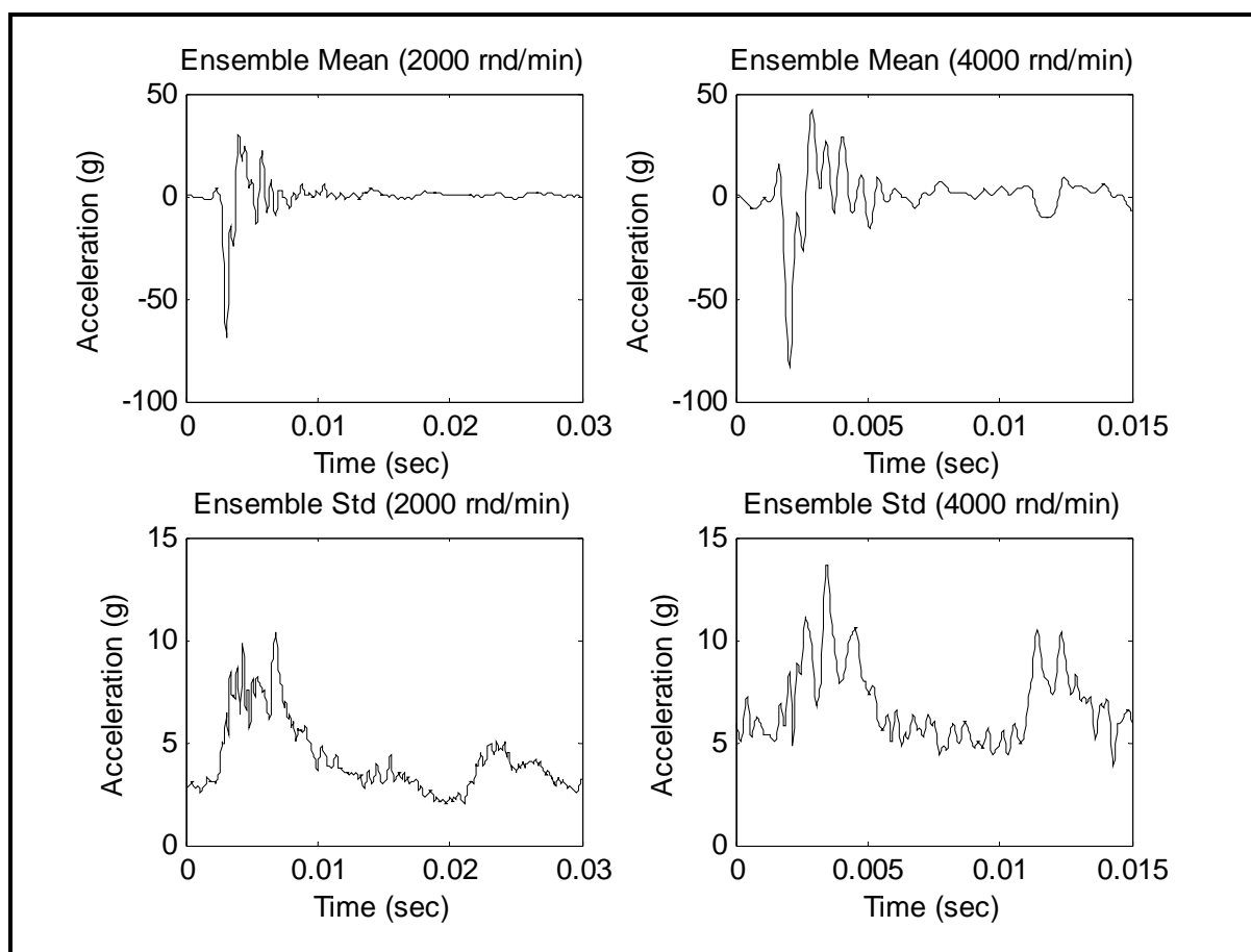
Figure 519.6B-4. Pre-processed gunfire shock measured time trace pulse ensemble statistics.
