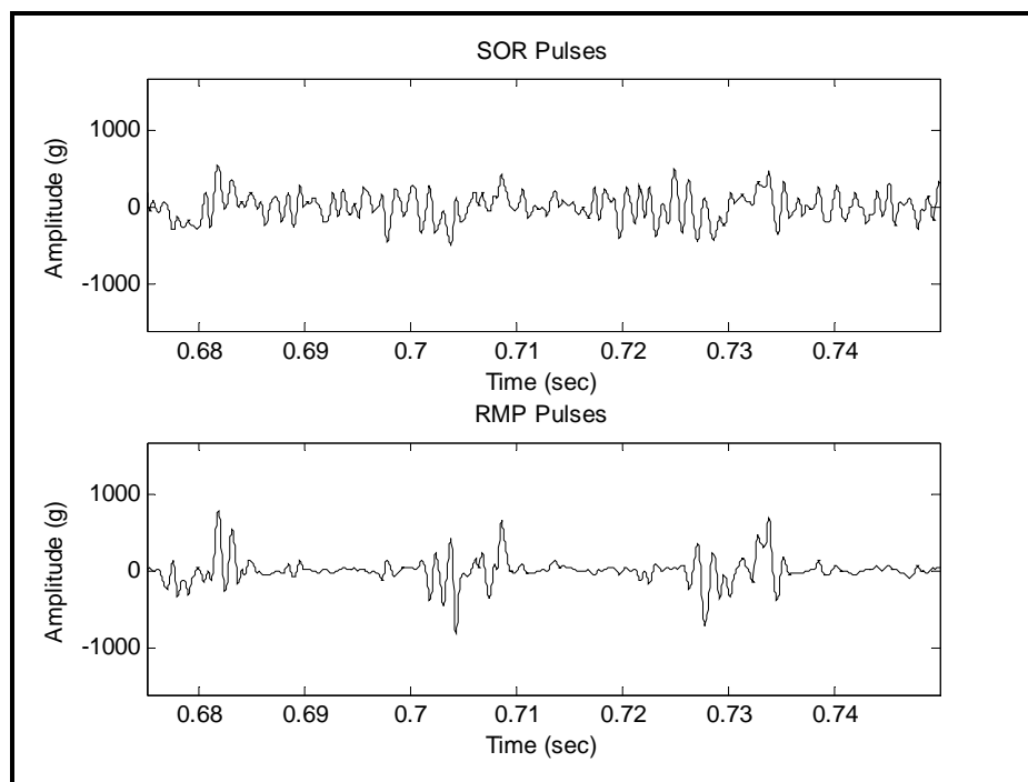
Figure 519.6C-6. High resolution sample model pulse train (three pulses).
